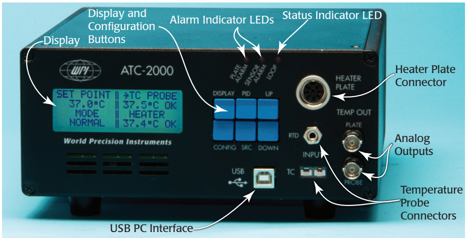
Fig. 5—Front panel of the ATC2000
